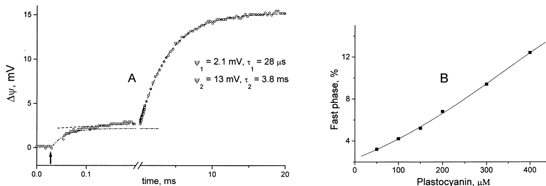
Fig. 3. Kinetics and relative contribution of the fast kinetic component of the \Delta\psi generation. A: Difference between the flash-induced photoelectric responses in the presence of 400 \mu M of Pc (Fig. 2A, trace 3) and in the absence of Pc (Fig. 2A, trace 1). B: Dependence of relative amplitude of the 30 \mu s kinetic component on Pc concentration. Conditions as in Fig. 1.
